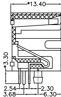
CUTAWAY VIEW
