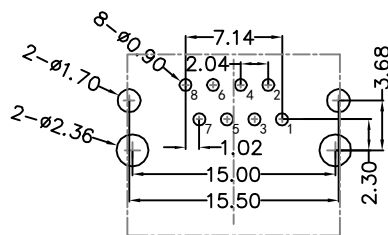
RECOMMENDED PCB LAYOUT VIEWED FROM COMPONENT SIDE
